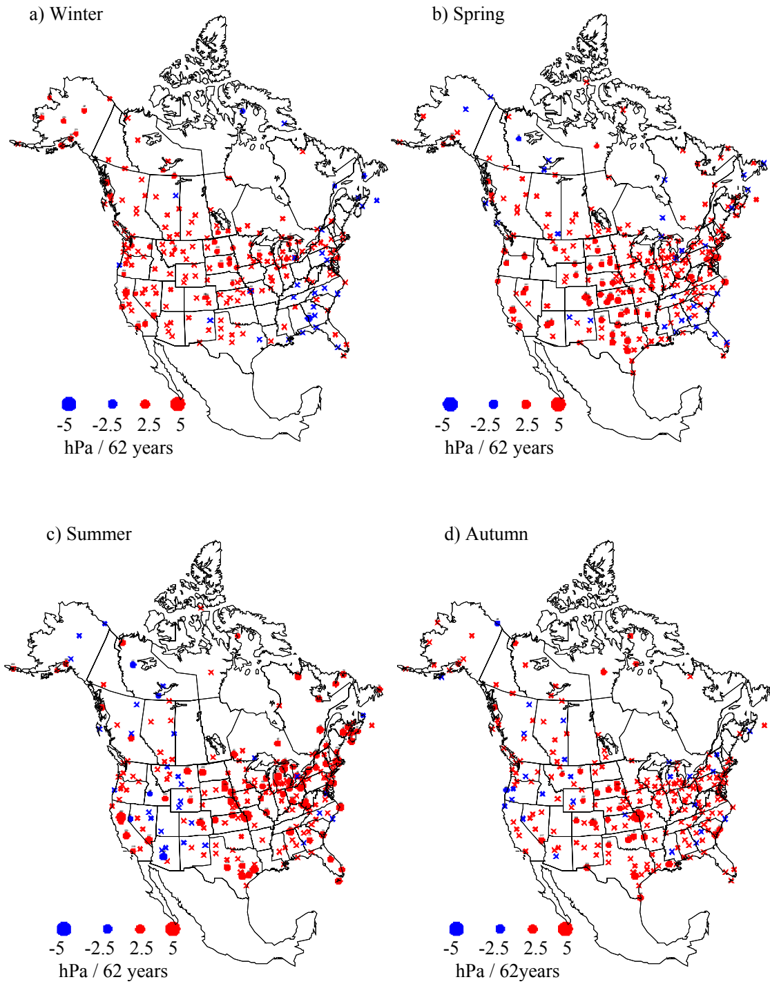
Fig. 5 Seasonal Dependence of Water Vapour Pressure Trends for 1948-2010. Crosses denote trends that are not statistically significant.
