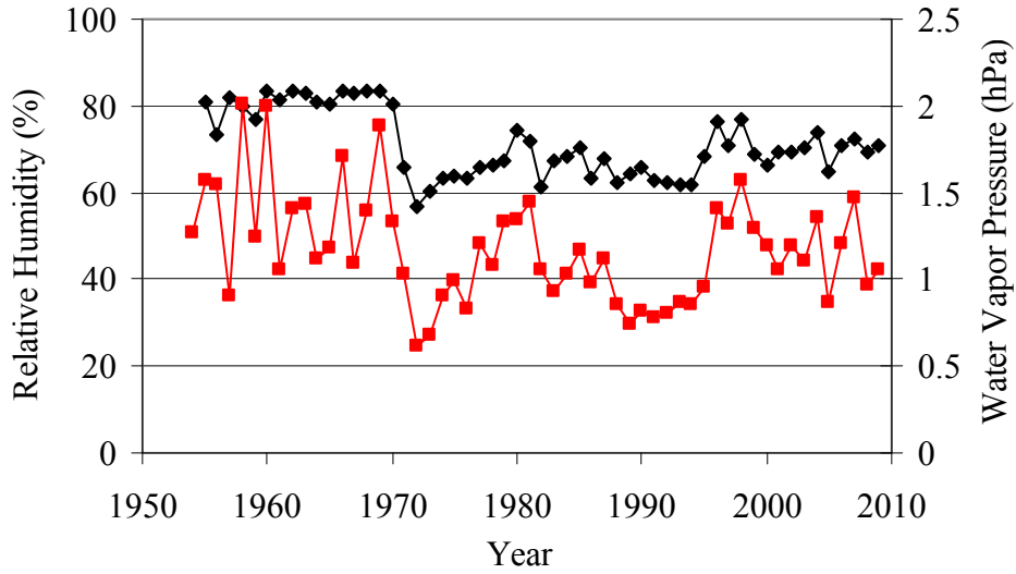
Fig. 1 Discontinuity of winter data for Schefferville, Quebec. Black dots denote Relative Humidity while red dots represent Water Vapour Pressure.
