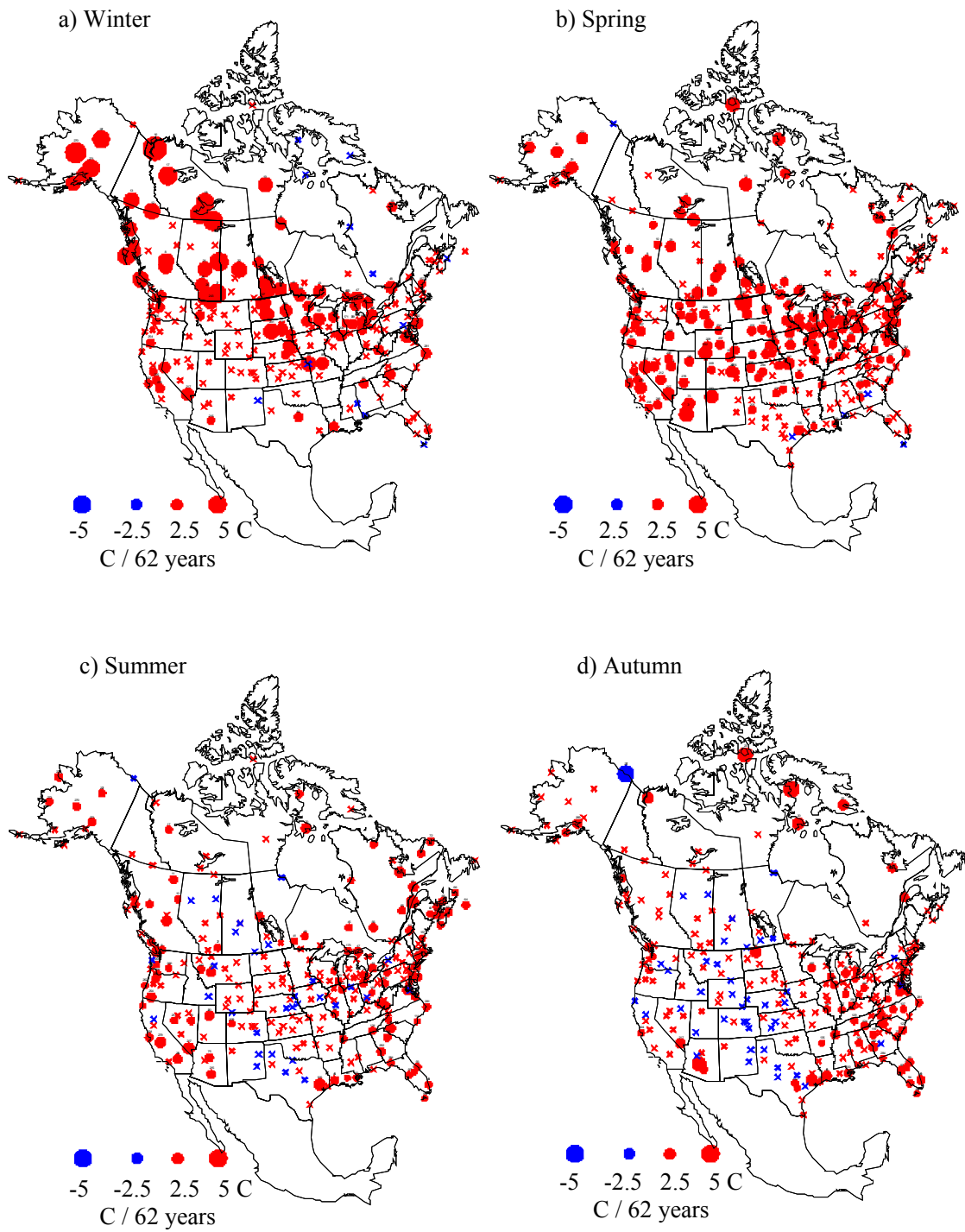
Fig. 4 Seasonal Dependence of Temperature Trends for 1948-2010. Crosses denote trends that are not statistically significant.
