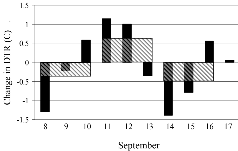
Fig. 7 Change in Diurnal Temperature Range averaged over stations located in the coterminous U.S. during Sept. 8 – 17, 2001 compared to the value during 1975-2005. The cross hatched bars denote the 3 day average values.
