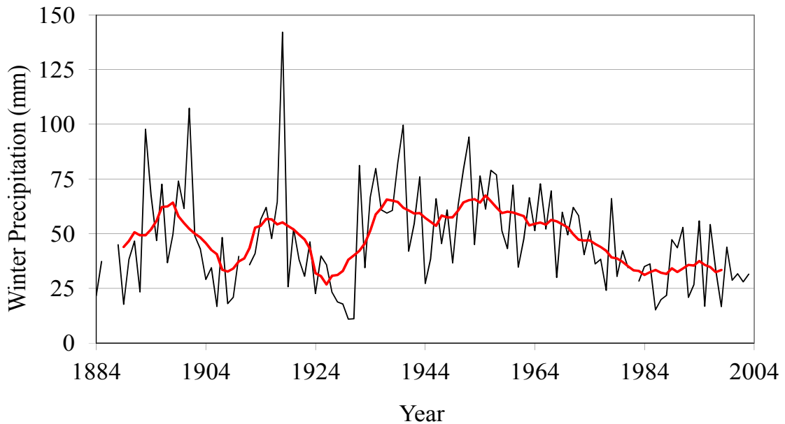
Fig. 2 Winter Precipitation at Medicine Hat, Alberta. The red line is the 5 year running average. This is computed using daily observations of precipitation that are available for a longer period of time than hourly measurements.
